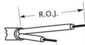
R.O.J., Cut Back and Strip
